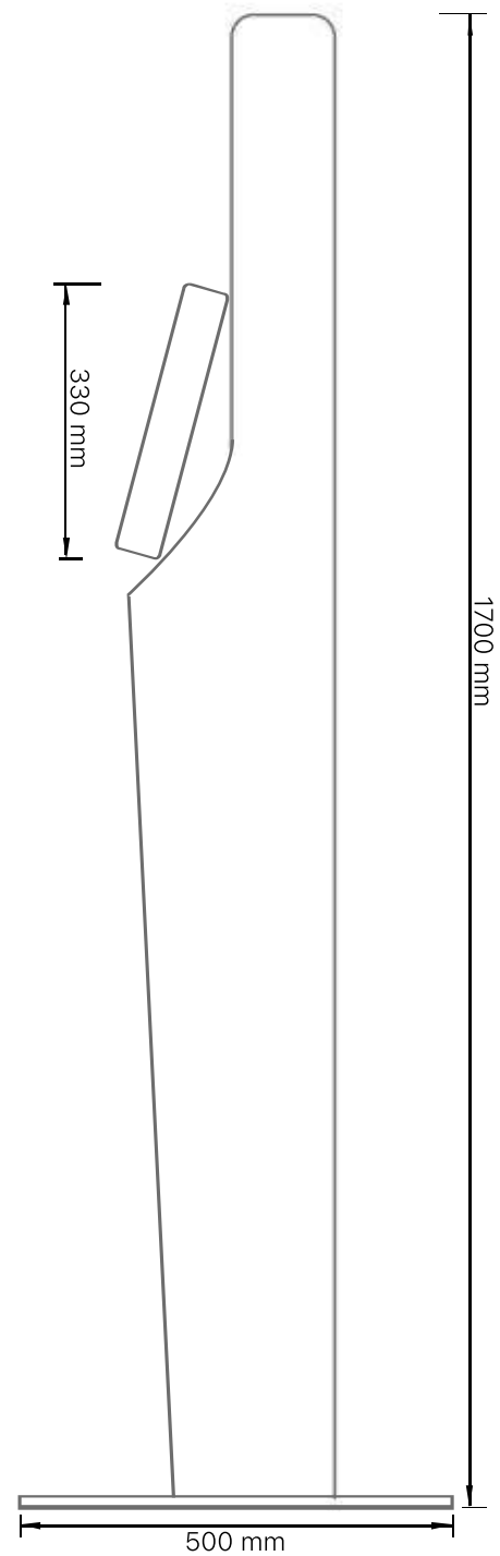
Side View
