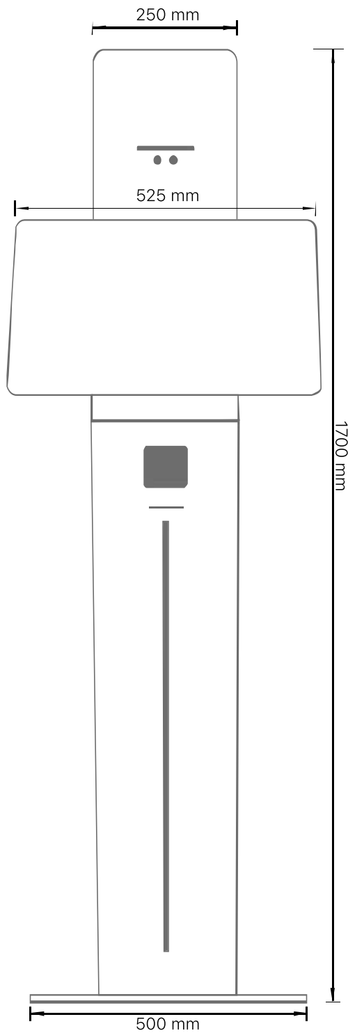
Front View
